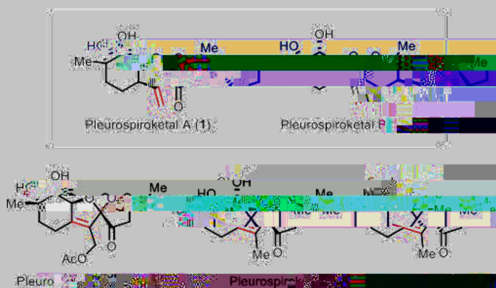
Figure 1. Structure of Pleurospiroketals
